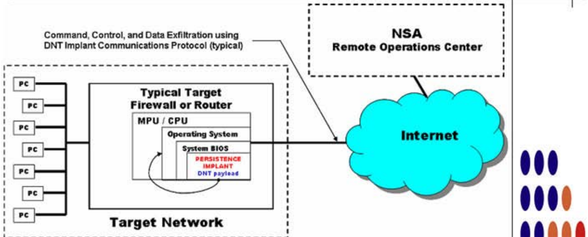
(S//SI//REL) STUCCOMONTANA Concept of Operations
